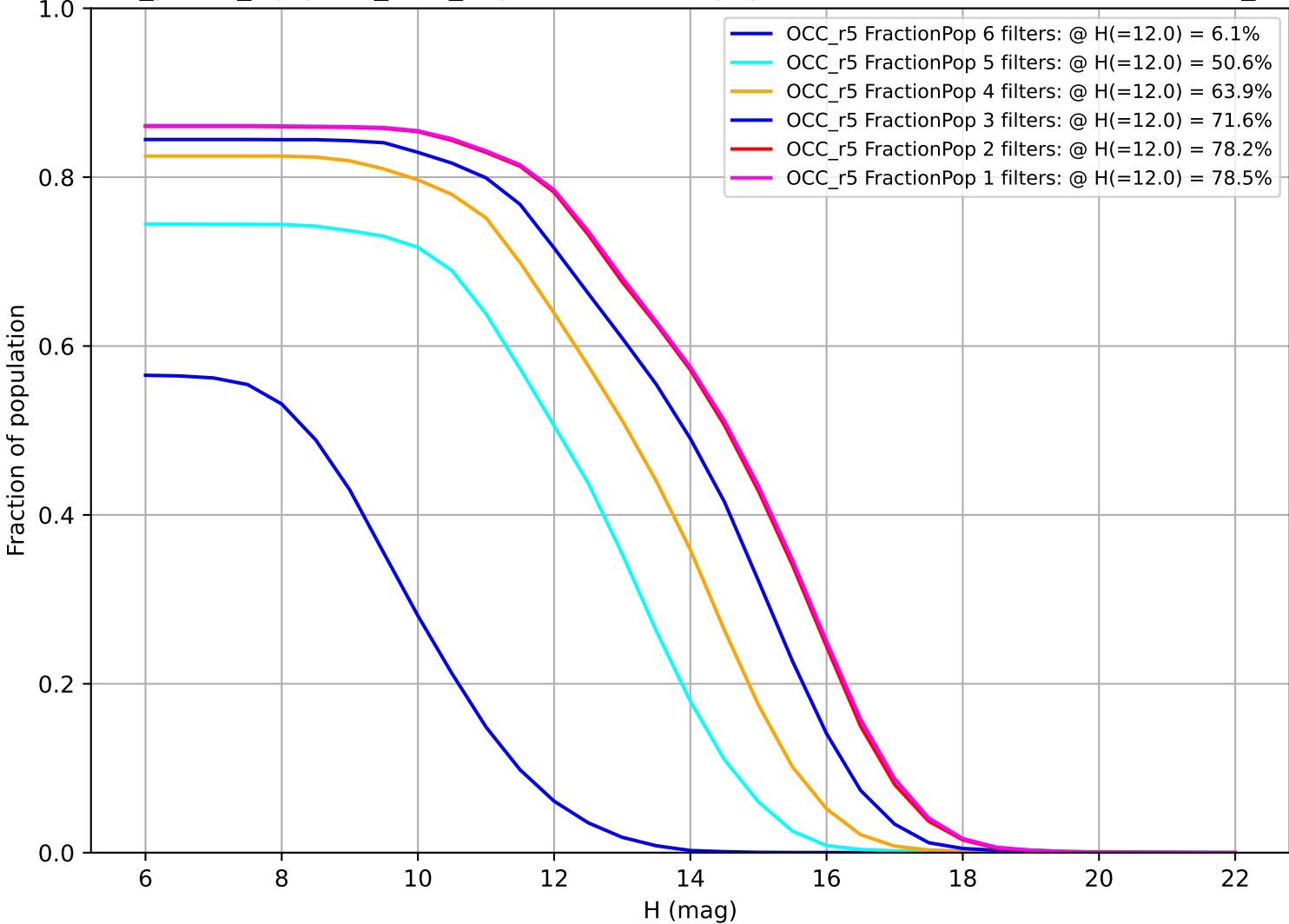
roll_pause_mjdp270_v3.4_10yrs: Fraction of population with colors in X filters OCC_r5
