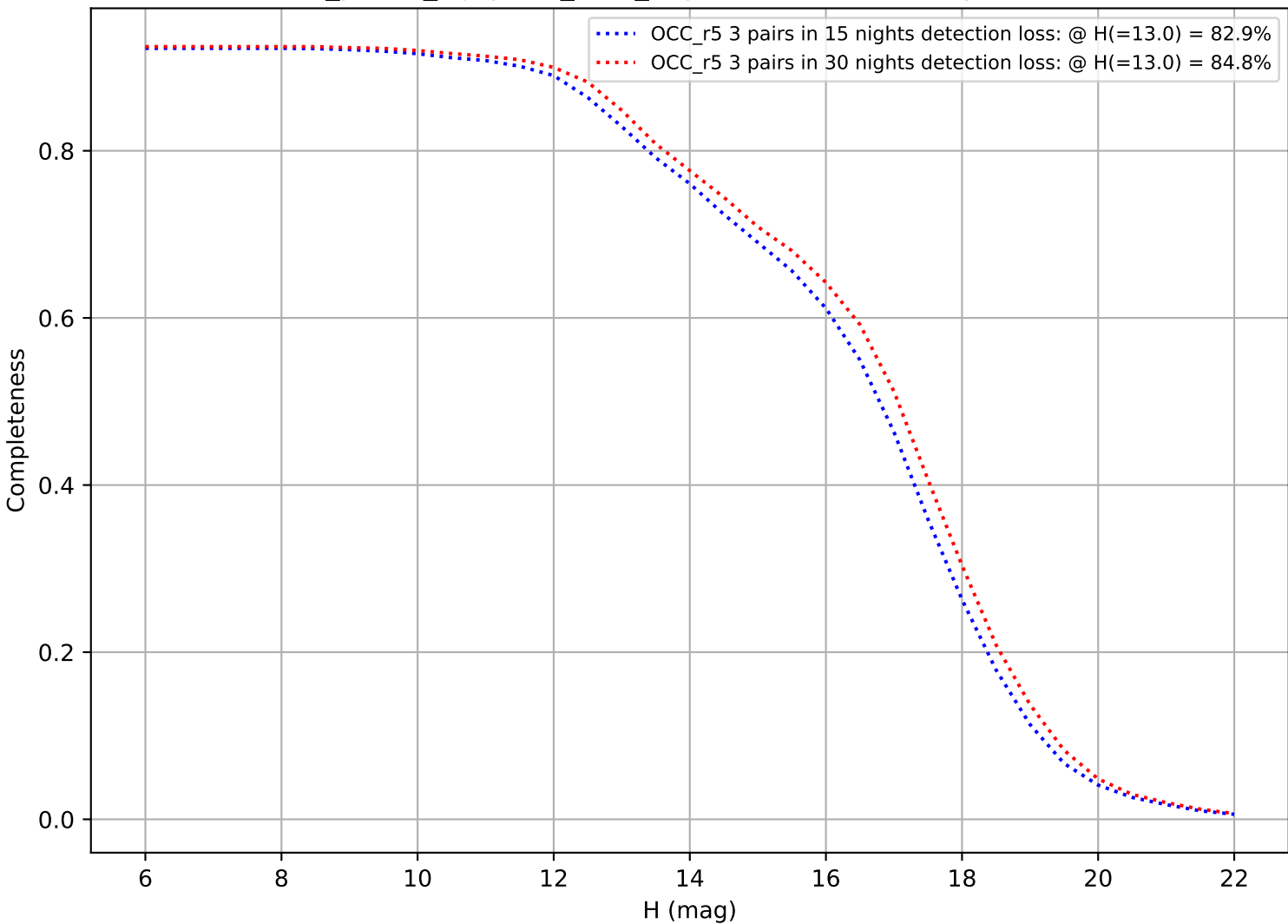
roll_pause_mjdp270_v3.4_10yrs: DifferentialCompleteness
