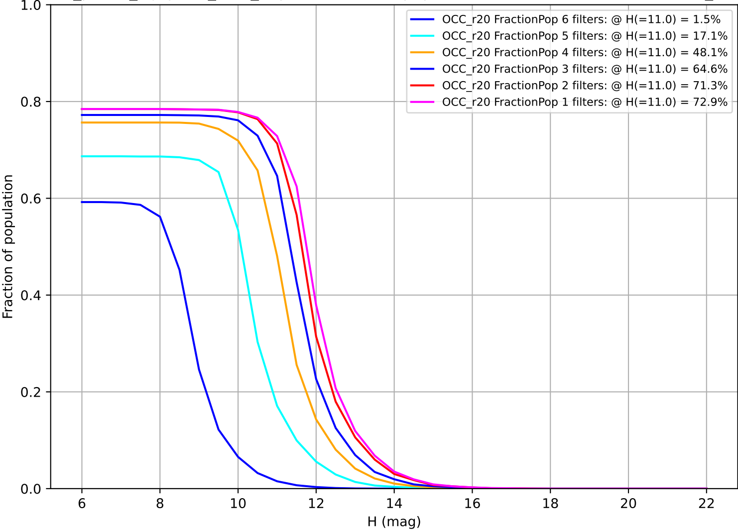
roll_pause_mjdp270_v3.4_10yrs: Fraction of population with colors in X filters OCC_r20
