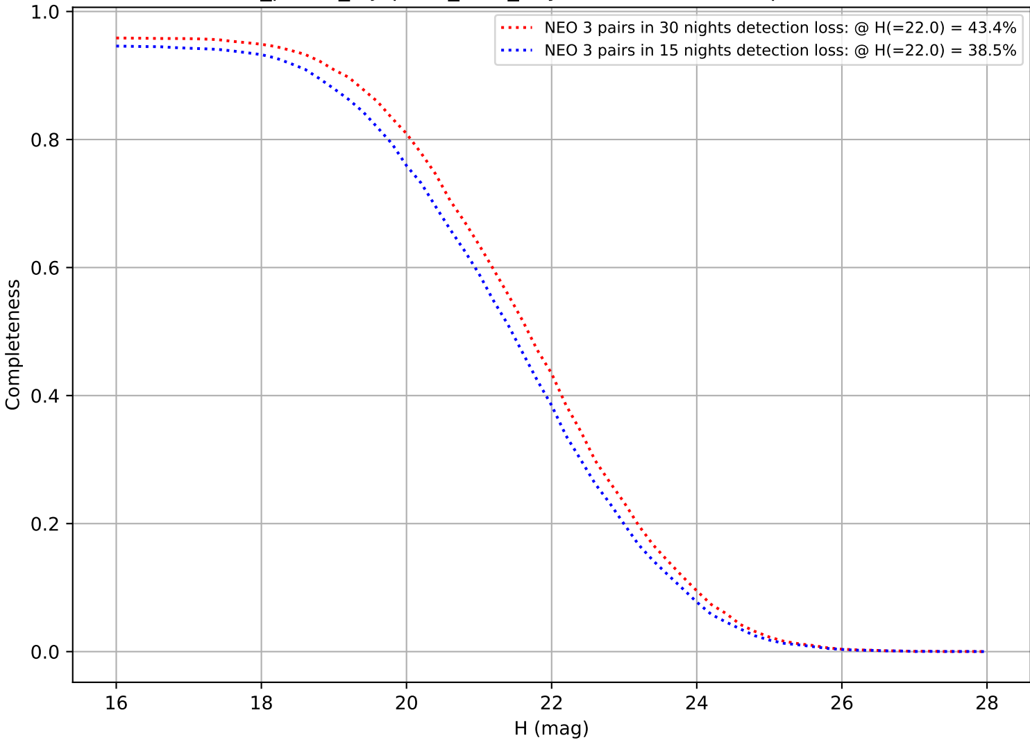
roll_pause_mjdp270_v3.4_10yrs: DifferentialCompleteness
