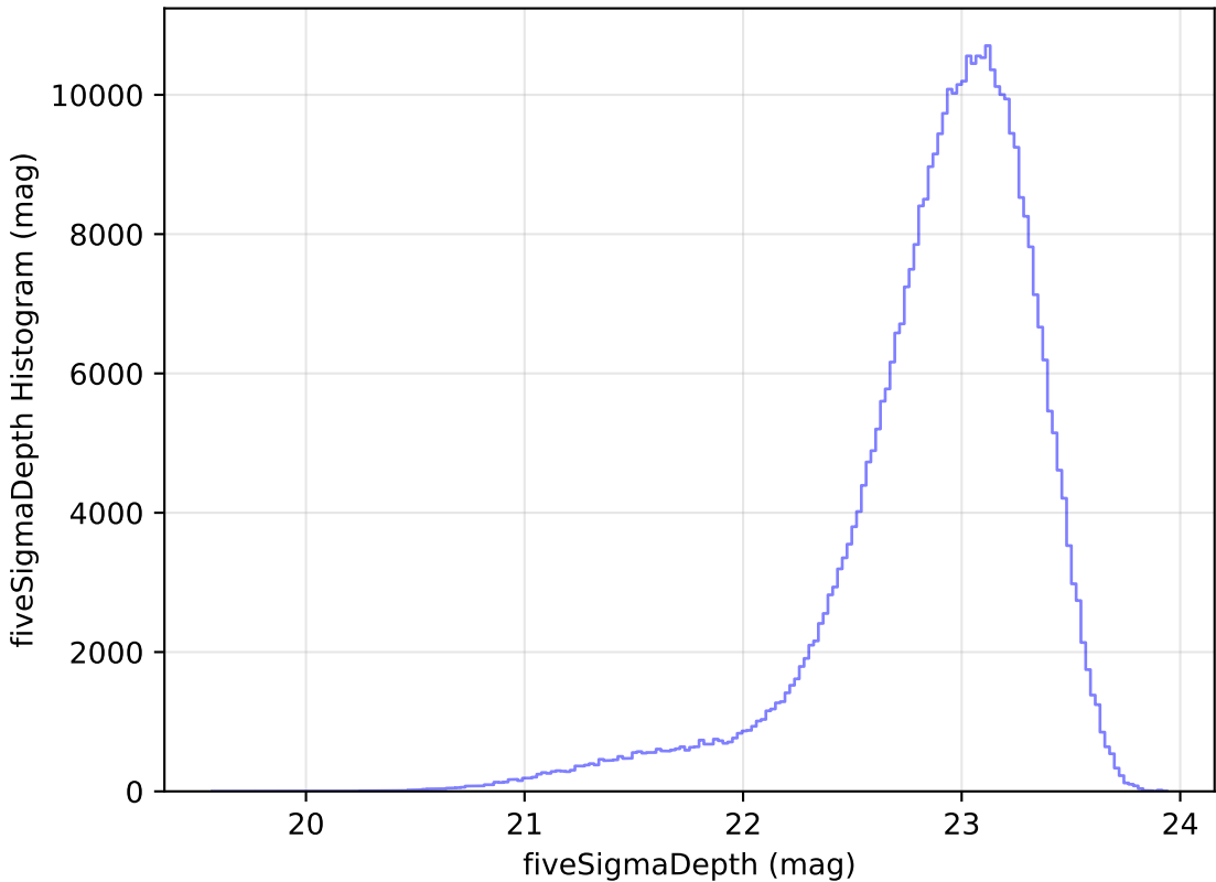
roll_pause_mjdp270_v3.4_10yrs z: fiveSigmaDepth Histogram
