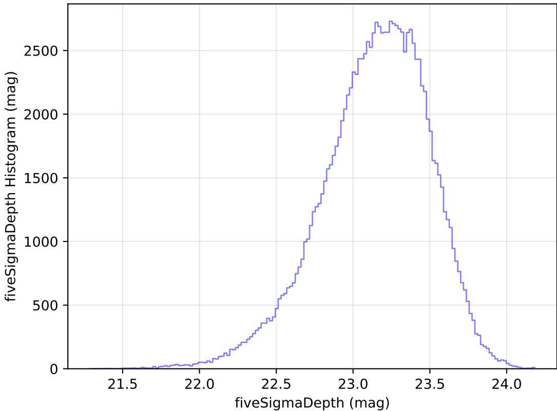
roll_pause_mjdp270_v3.4_10yrs u: fiveSigmaDepth Histogram
