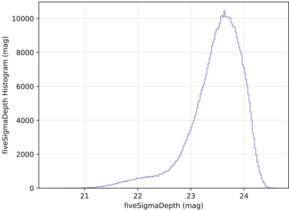
roll_pause_mjdp270_v3.4_10yrs i: fiveSigmaDepth Histogram
