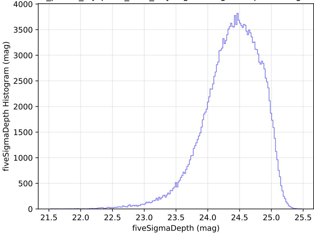
roll_pause_mjdp270_v3.4_10yrs g: fiveSigmaDepth Histogram
