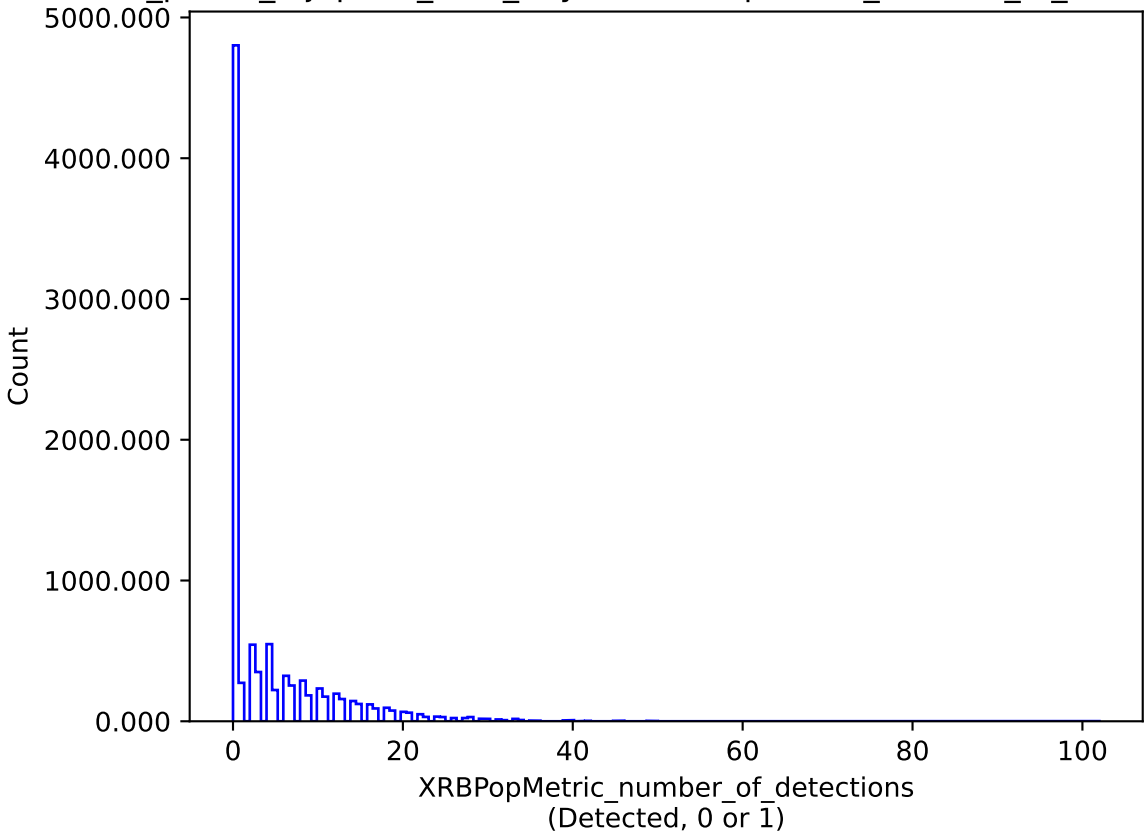
roll_pause_mjdp270_v3.4_10yrs : XRBPopMetric_number_of_detections
