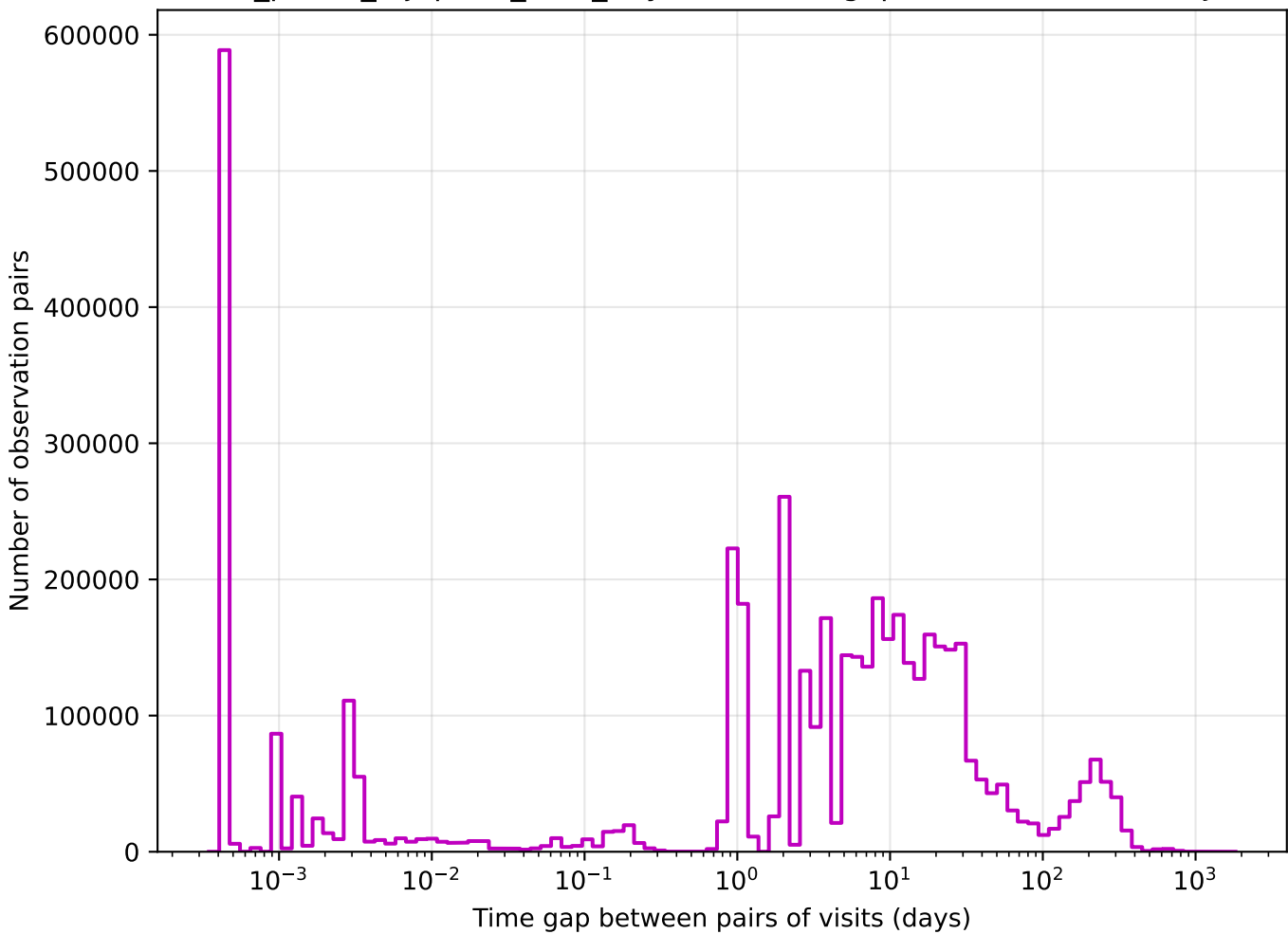
roll_pause_mjdp270_v3.4_10yrs z band: Tgaps observationStartMJD
