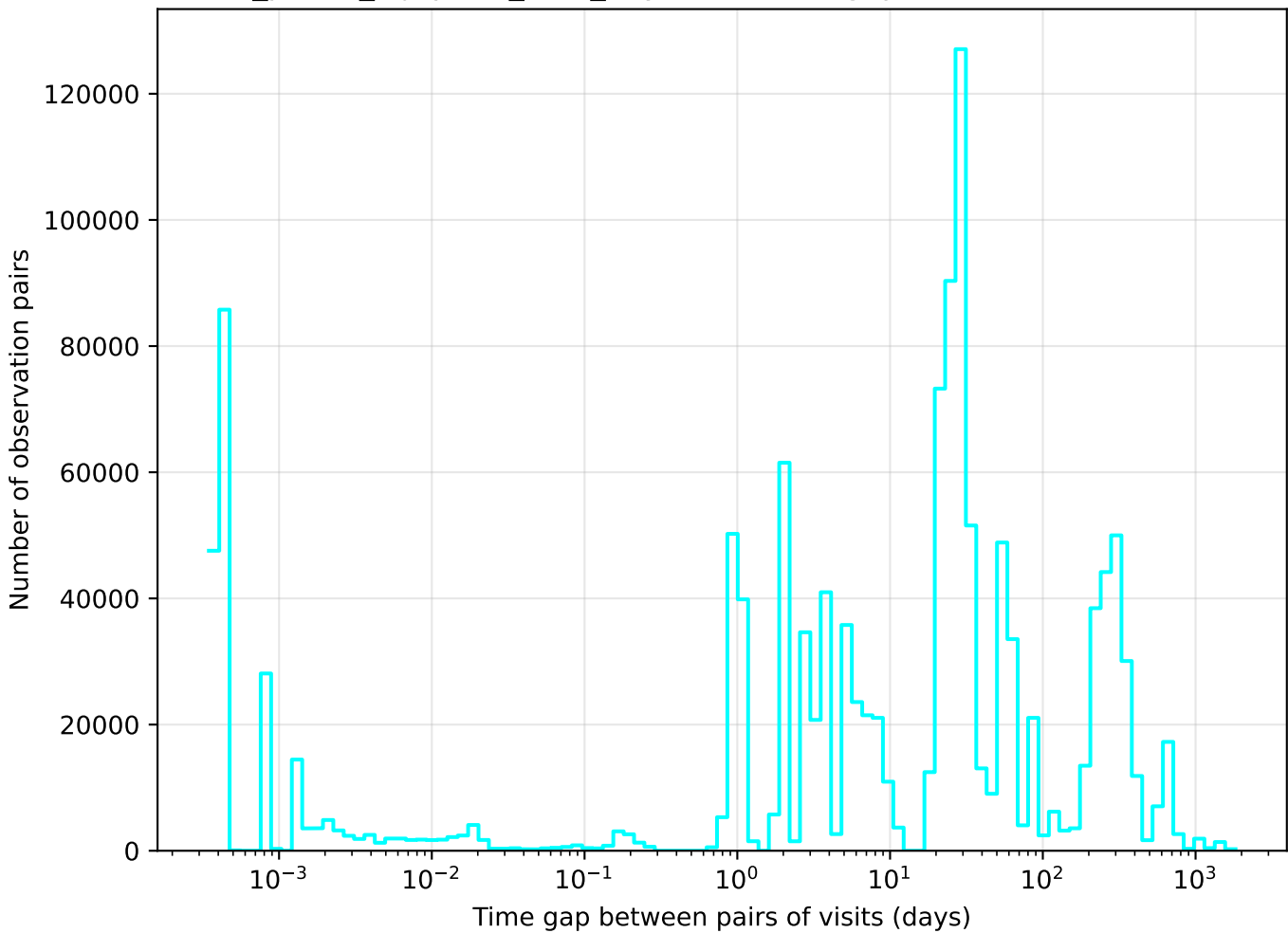
roll_pause_mjdp270_v3.4_10yrs u band: Tgaps observationStartMJD
