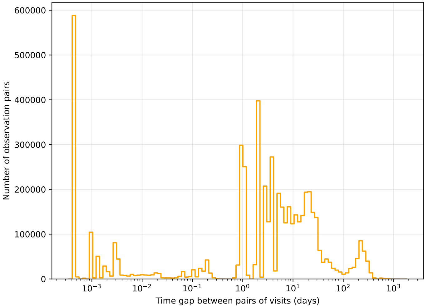
roll_pause_mjdp270_v3.4_10yrs r band: Tgaps observationStartMJD
