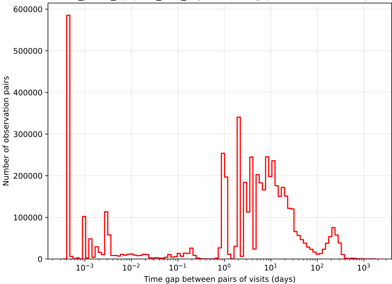
roll_pause_mjdp270_v3.4_10yrs i band: Tgaps observationStartMJD
