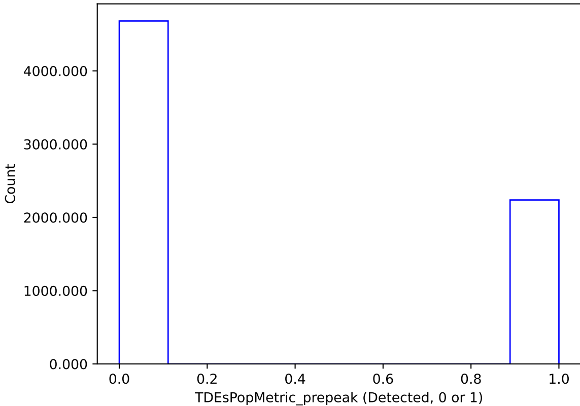
roll_pause_mjdp270_v3.4_10yrs : TDEsPopMetric_prepeak
