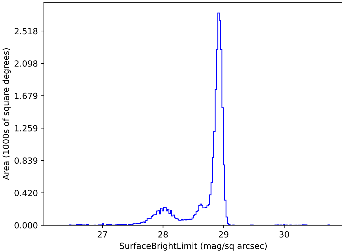
roll_pause_mjdp270_v3.4_10yrs u: SurfaceBrightLimit
