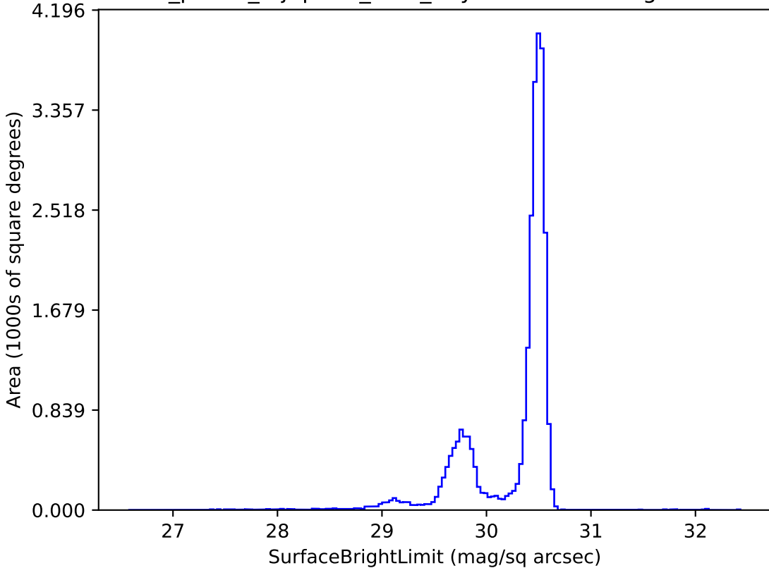
roll_pause_mjdp270_v3.4_10yrs r: SurfaceBrightLimit
