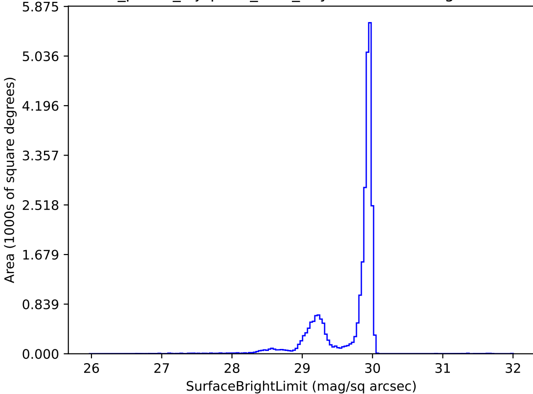
roll_pause_mjdp270_v3.4_10yrs i: SurfaceBrightLimit
