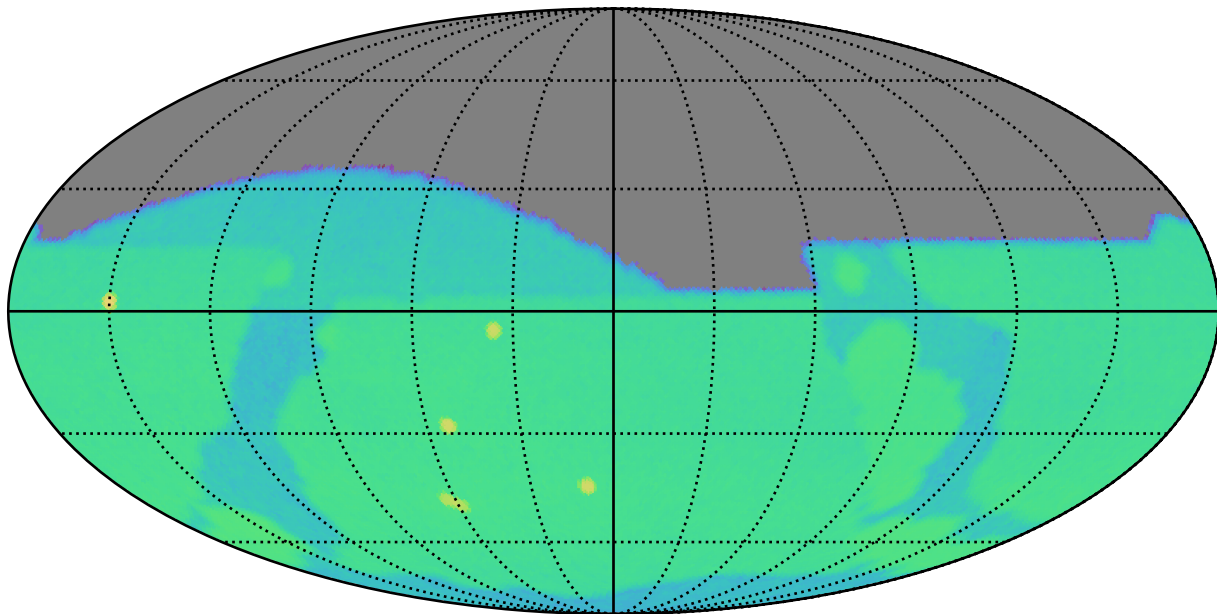
roll_pause_mjdp270_v3.4_10yrs g: SurfaceBrightLimit
