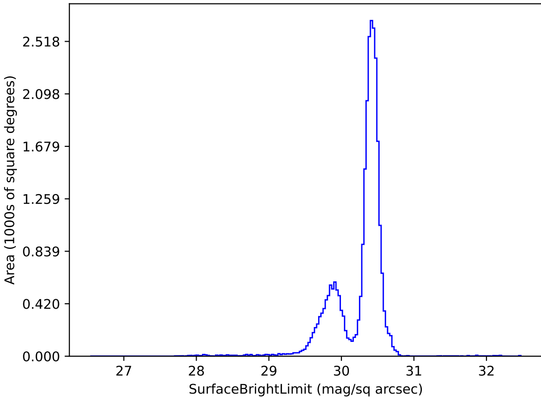
roll_pause_mjdp270_v3.4_10yrs g: SurfaceBrightLimit
