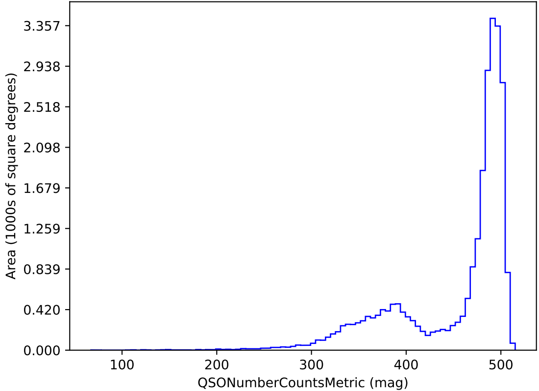
roll_pause_mjdp270_v3.4_10yrs z band and non-DD: QSONumberCountsMetric
