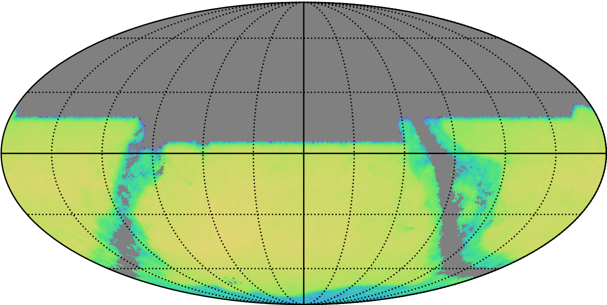
roll_pause_mjdp270_v3.4_10yrs y band and non-DD: QSONumberCountsMetric
