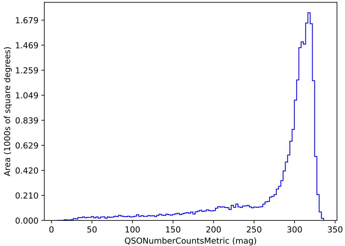
roll_pause_mjdp270_v3.4_10yrs u band and non-DD: QSONumberCountsMetric
