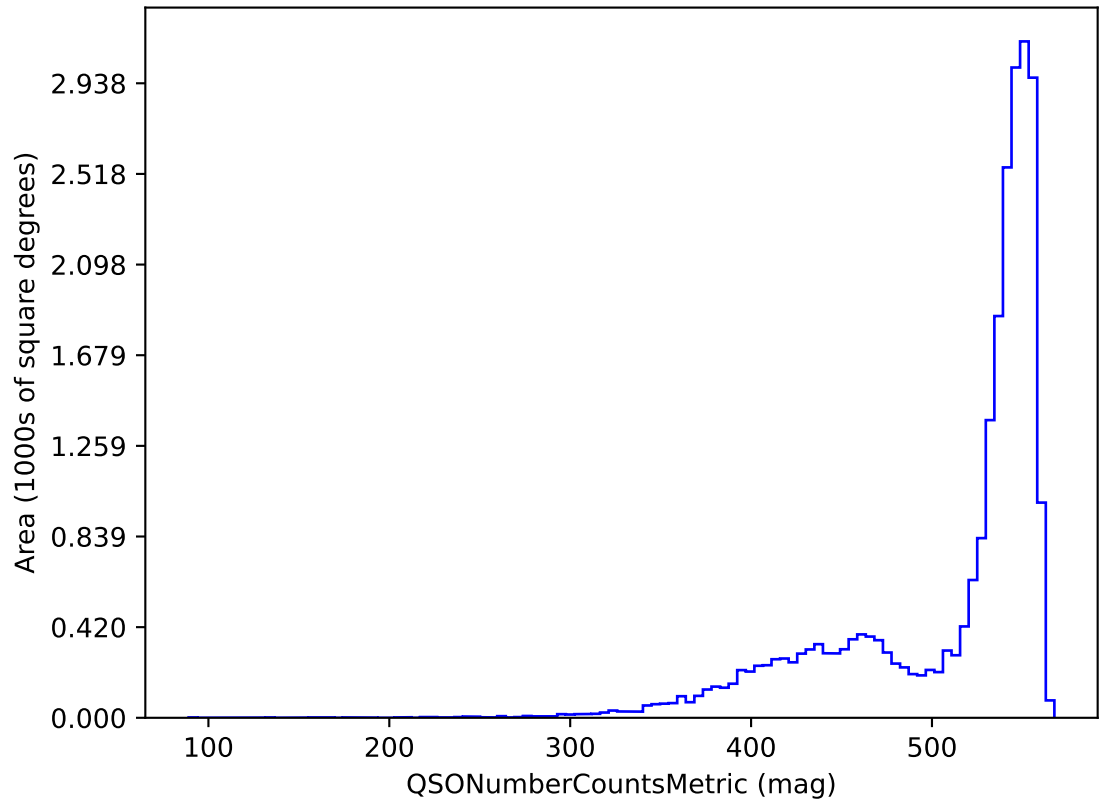
roll_pause_mjdp270_v3.4_10yrs i band and non-DD: QSONumberCountsMetric
