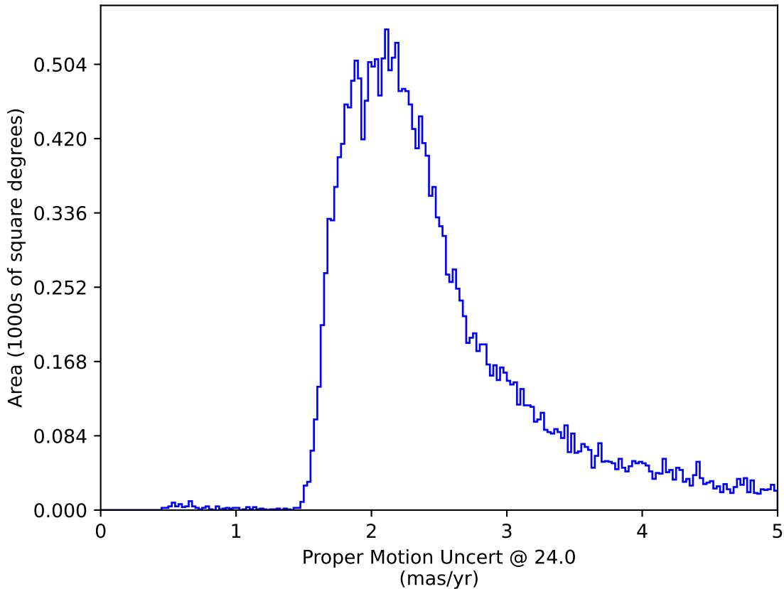
roll_pause_mjdp270_v3.4_10yrs : Proper Motion Uncert @ 24.0
