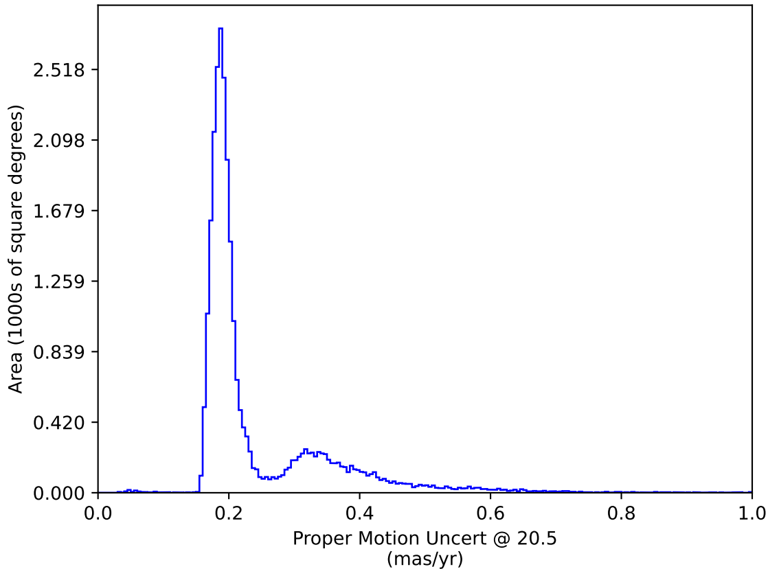
roll_pause_mjdp270_v3.4_10yrs : Proper Motion Uncert @ 20.5
