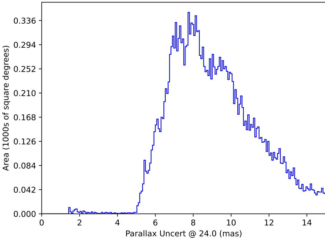
roll_pause_mjdp270_v3.4_10yrs : Parallax Uncert @ 24.0
