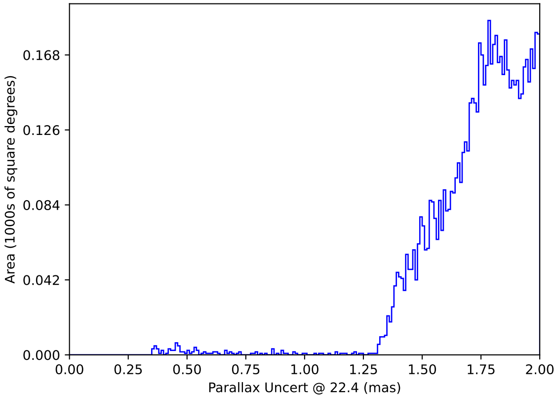
roll_pause_mjdp270_v3.4_10yrs : Parallax Uncert @ 22.4
