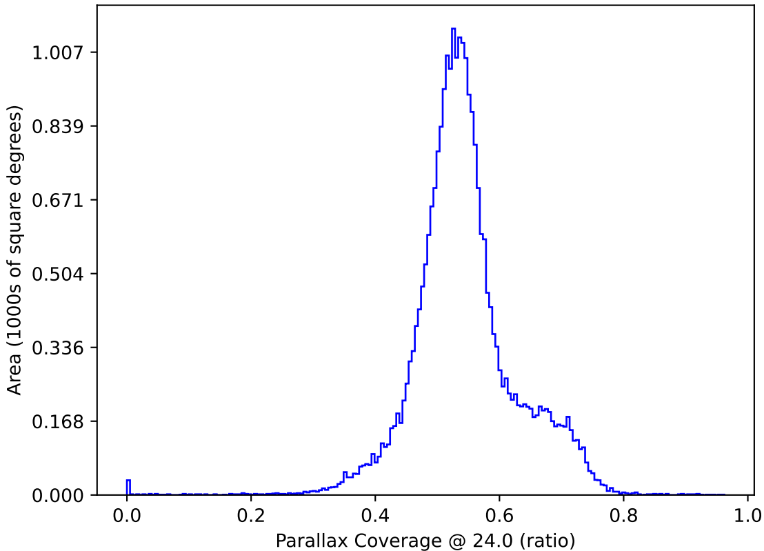
roll_pause_mjdp270_v3.4_10yrs : Parallax Coverage @ 24.0
