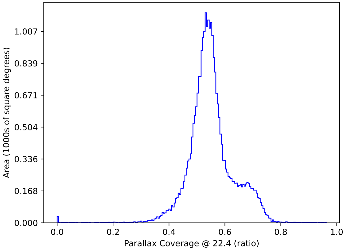
roll_pause_mjdp270_v3.4_10yrs : Parallax Coverage @ 22.4
