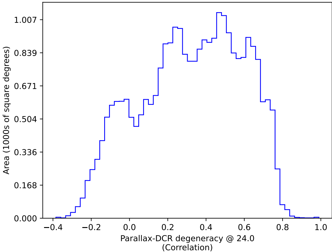
roll_pause_mjdp270_v3.4_10yrs : Parallax-DCR degeneracy @ 24.0
