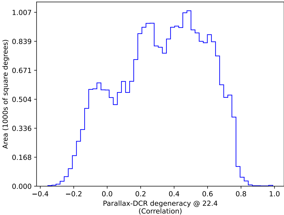
roll_pause_mjdp270_v3.4_10yrs : Parallax-DCR degeneracy @ 22.4
