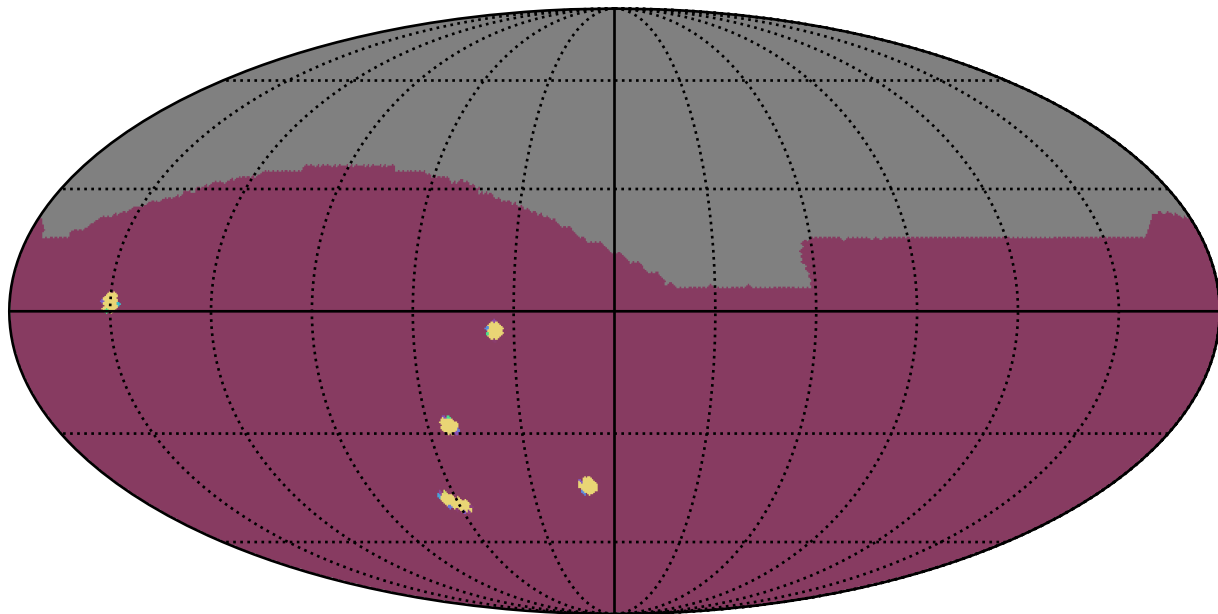
roll_pause_mjdp270_v3.4_10yrs : NumberOfQuickRevisits
