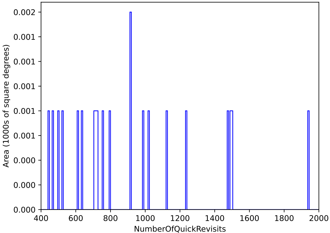
roll_pause_mjdp270_v3.4_10yrs : NumberOfQuickRevisits
