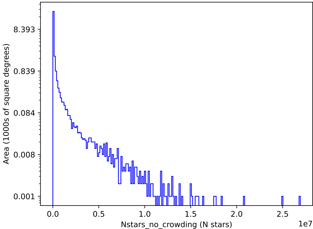
roll_pause_mjdp270_v3.4_10yrs z: Nstars_no_crowding
