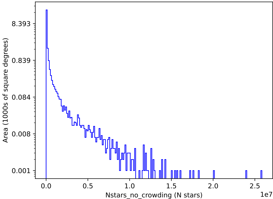
roll_pause_mjdp270_v3.4_10yrs y: Nstars_no_crowding
