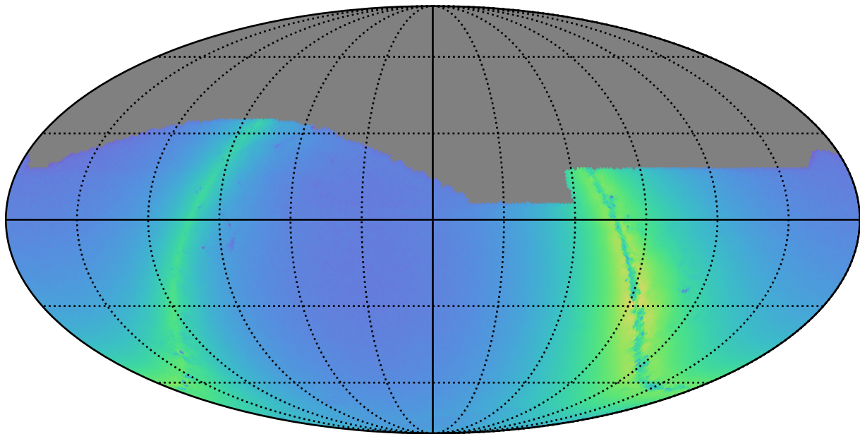
roll_pause_mjdp270_v3.4_10yrs i: Nstars_no_crowding
