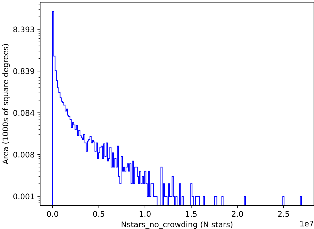
roll_pause_mjdp270_v3.4_10yrs i: Nstars_no_crowding
