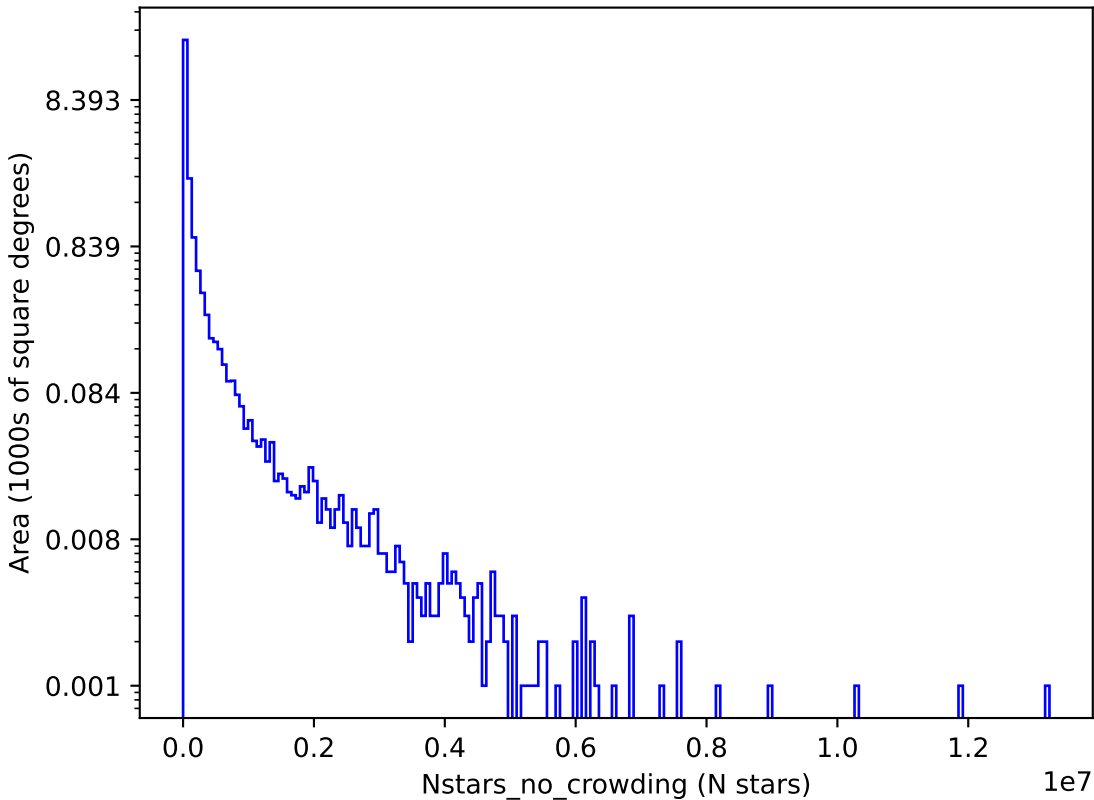
roll_pause_mjdp270_v3.4_10yrs g: Nstars_no_crowding
