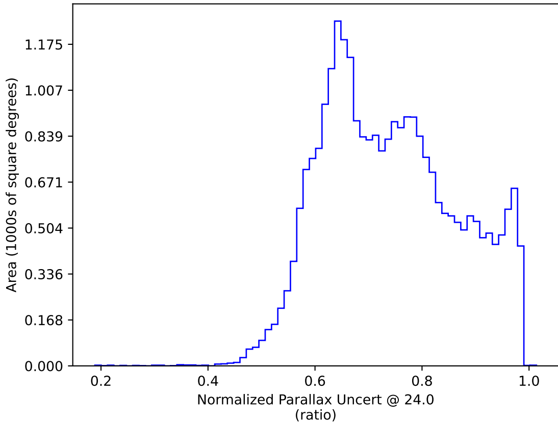
roll_pause_mjdp270_v3.4_10yrs : Normalized Parallax Uncert @ 24.0
