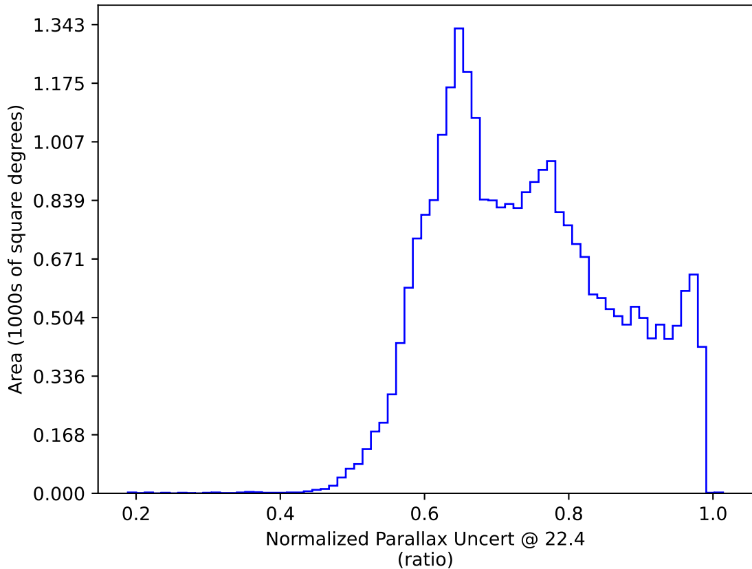
roll_pause_mjdp270_v3.4_10yrs : Normalized Parallax Uncert @ 22.4
