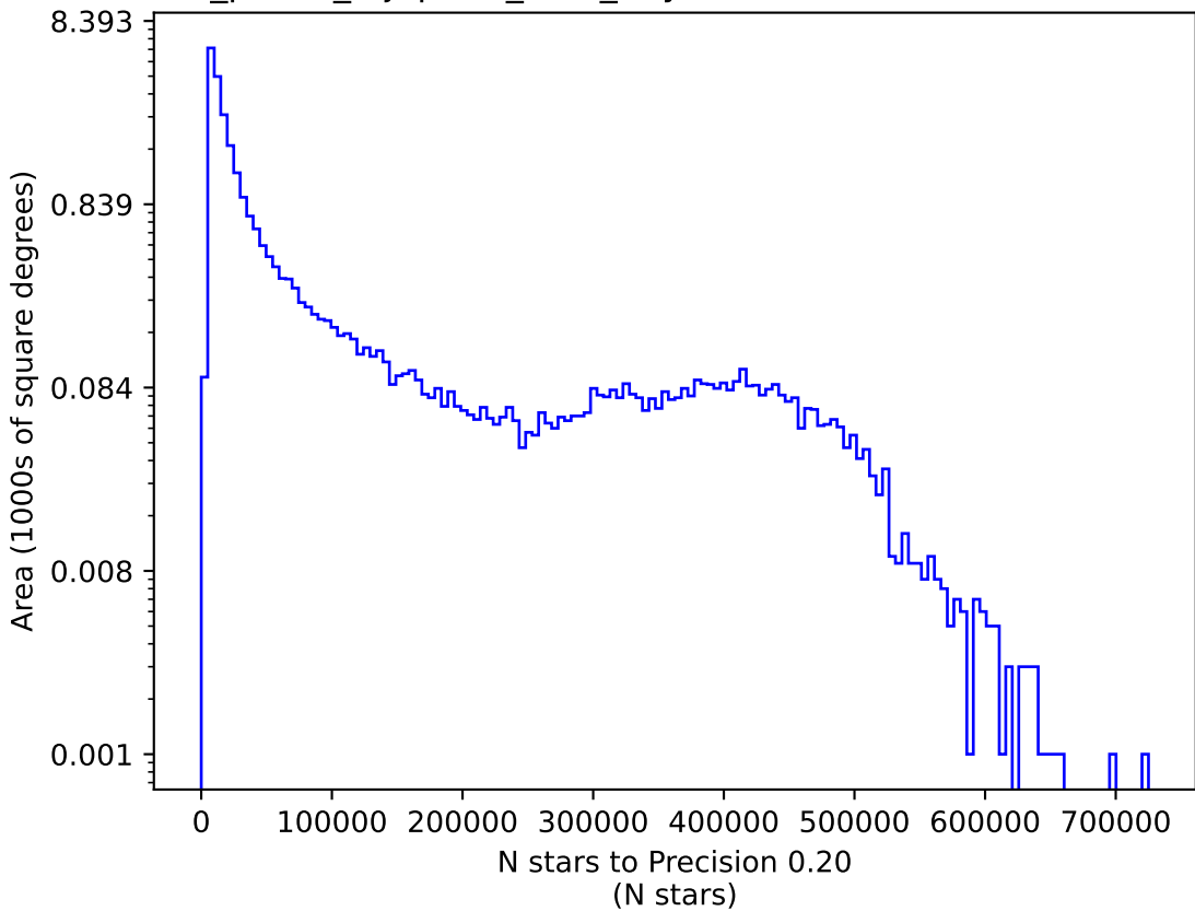
roll_pause_mjdp270_v3.4_10yrs z: N stars to Precision 0.20
