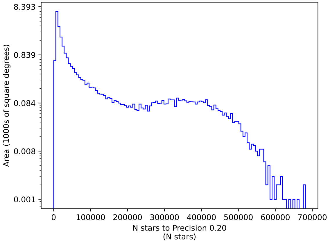
roll_pause_mjdp270_v3.4_10yrs y: N stars to Precision 0.20
