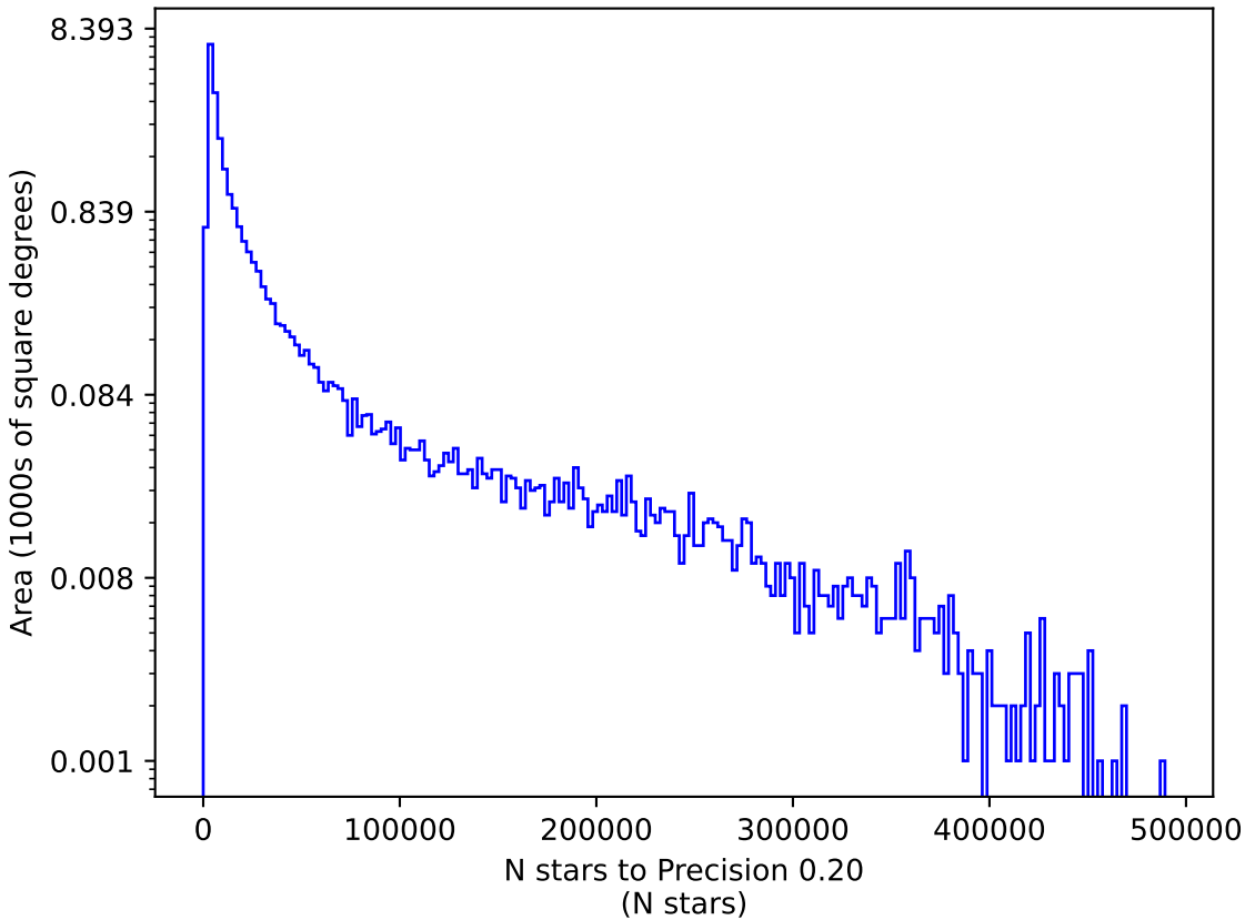
roll_pause_mjdp270_v3.4_10yrs u: N stars to Precision 0.20
