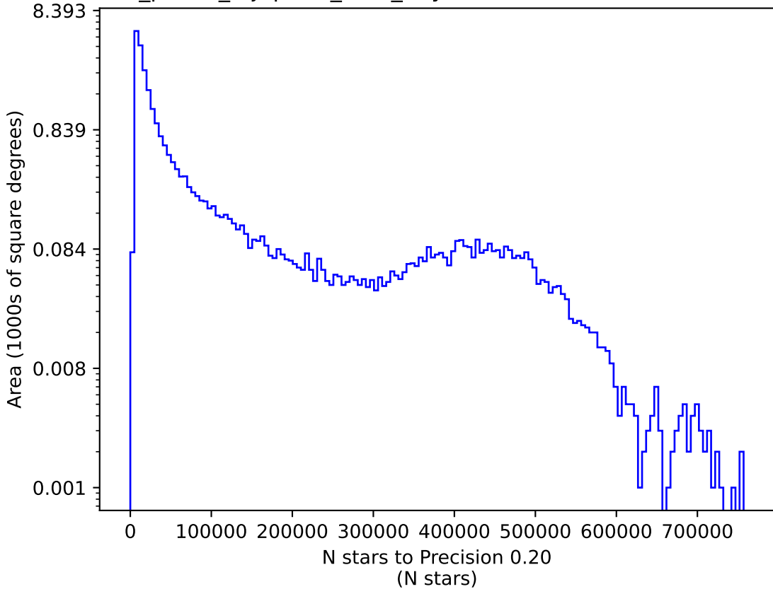
roll_pause_mjdp270_v3.4_10yrs i: N stars to Precision 0.20
