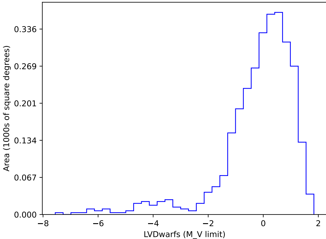
roll_pause_mjdp270_v3.4_10yrs gi SCP: LVDwarfs
