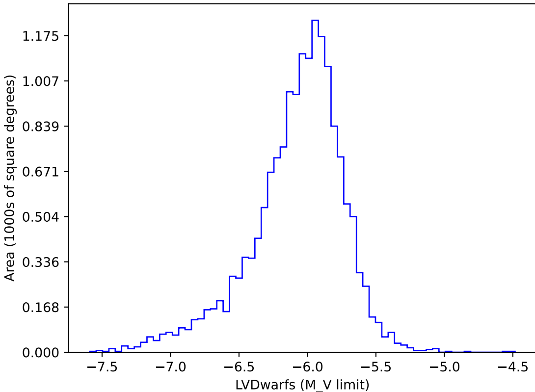
roll_pause_mjdp270_v3.4_10yrs gi: LVDwarfs
