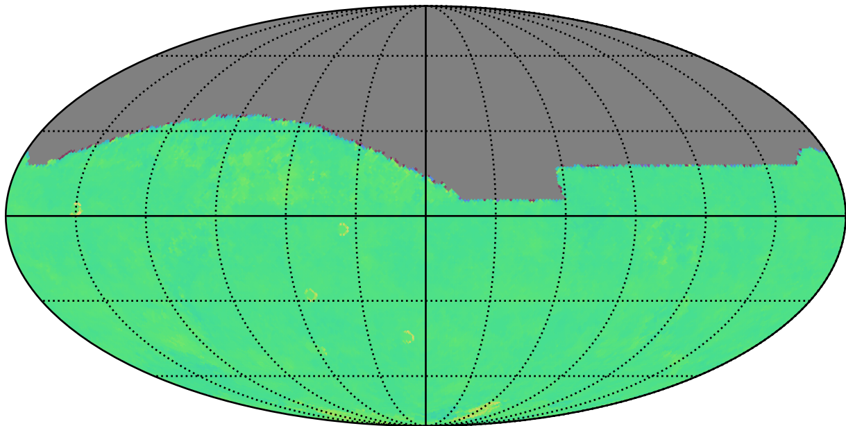
roll_pause_mjdp270_v3.4_10yrs z: Kuiper rotTelPos
