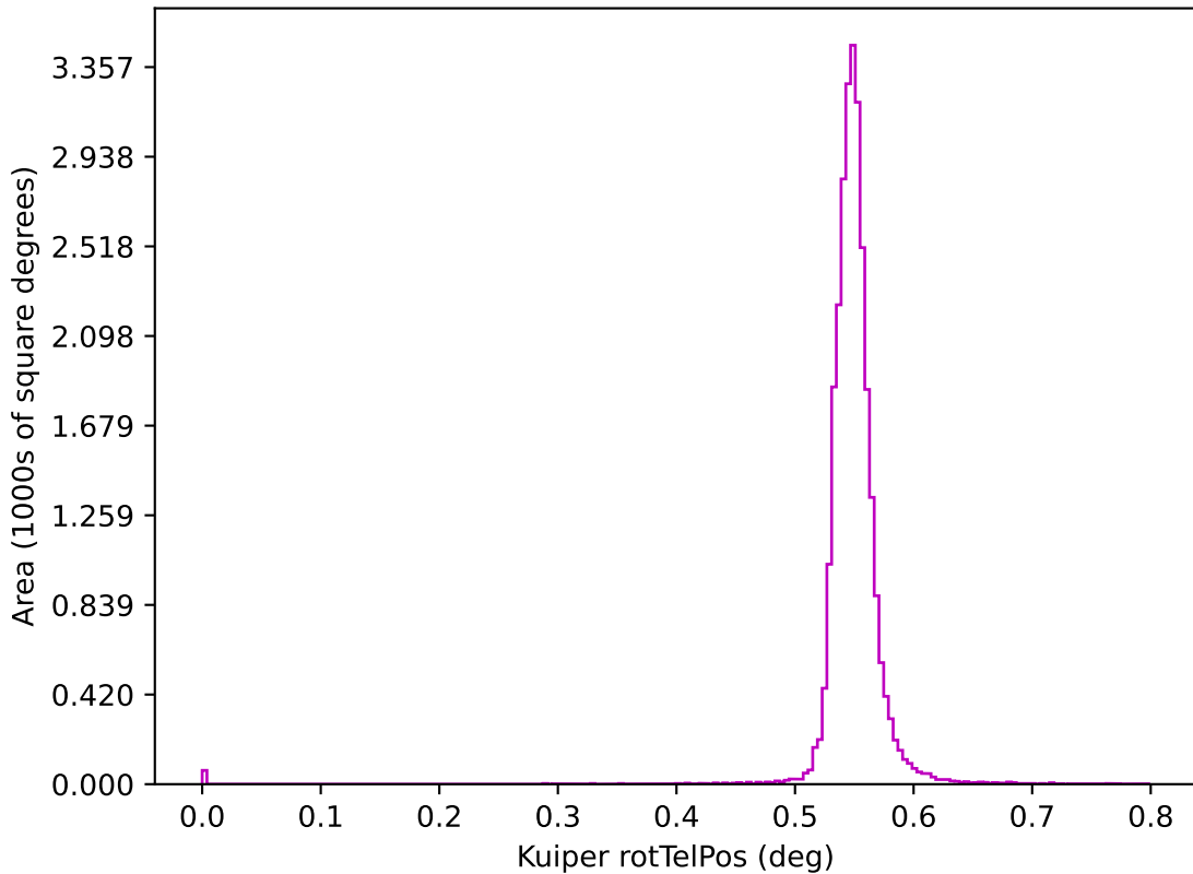
roll_pause_mjdp270_v3.4_10yrs z: Kuiper rotTelPos
