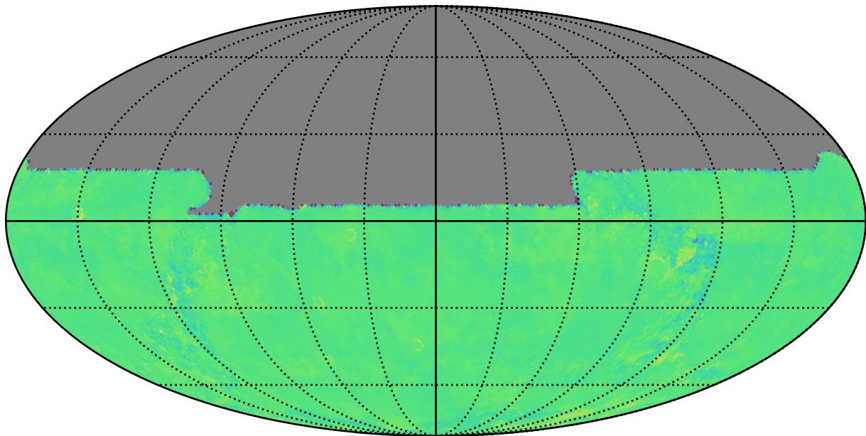
roll_pause_mjdp270_v3.4_10yrs u: Kuiper rotTelPos
