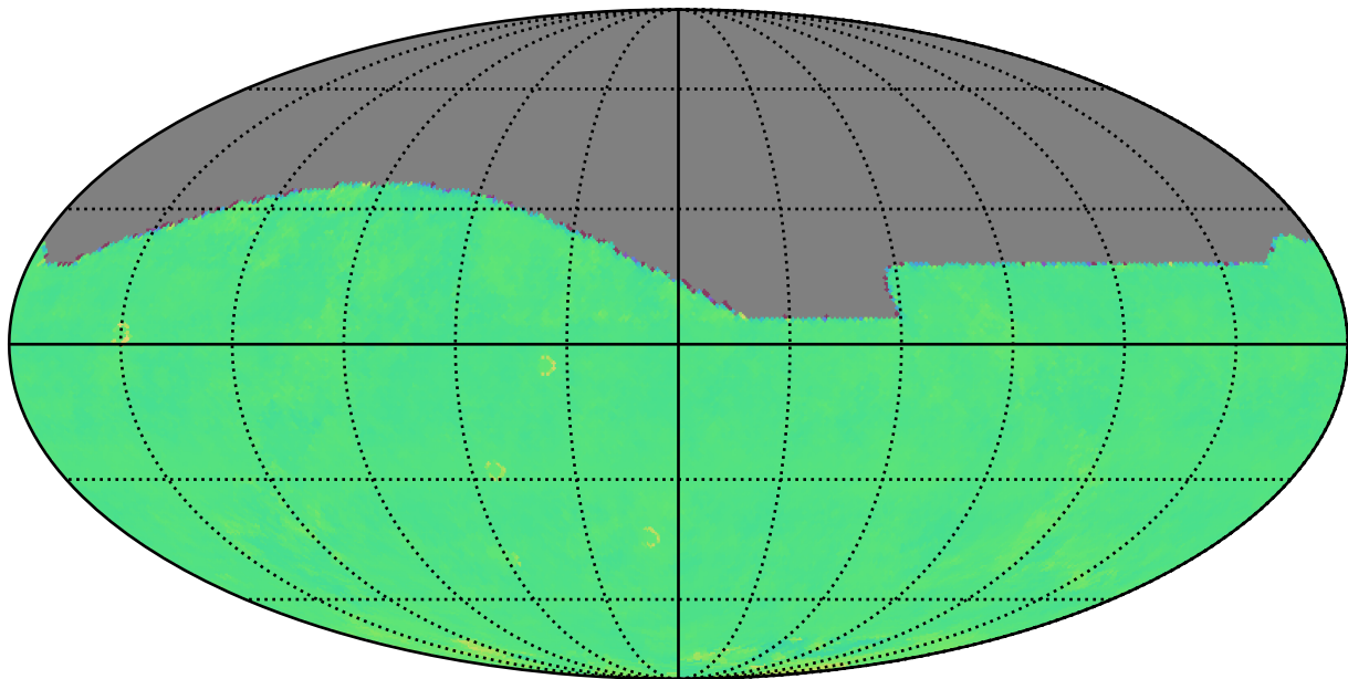
roll_pause_mjdp270_v3.4_10yrs r: Kuiper rotTelPos
